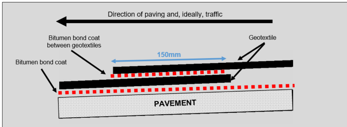
Figure 8.7.4.1 – Geotextile overlaps
